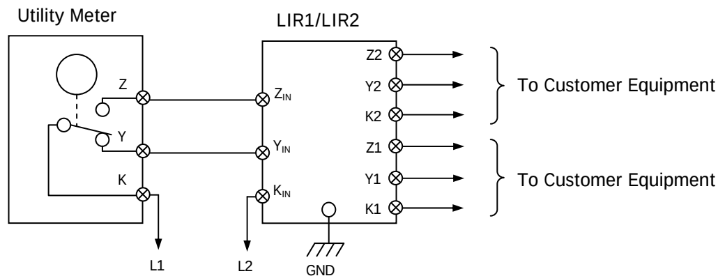
FIGURE 1: Wiring Diagram
